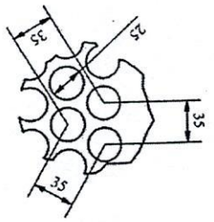
A (1:5)
